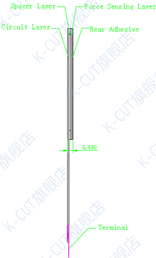
SIDE VIEW (NO SCALE)
